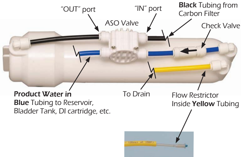
Fig. 2: Installation of ASO and Check Valve For Single Membrane Systems
