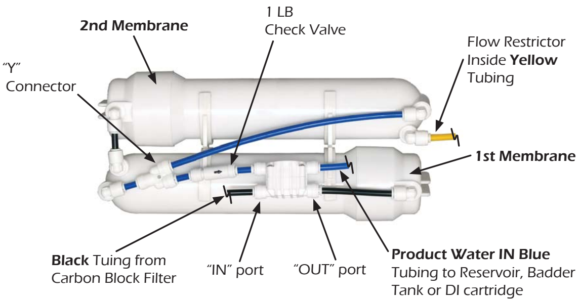
Fig. 3: Installation of ASO and Check Valve Back View of Dual Membrane Systems
