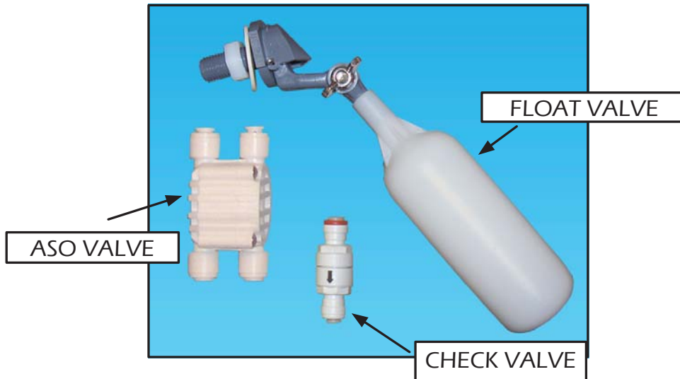
Fig. 1: ASOFK Components
