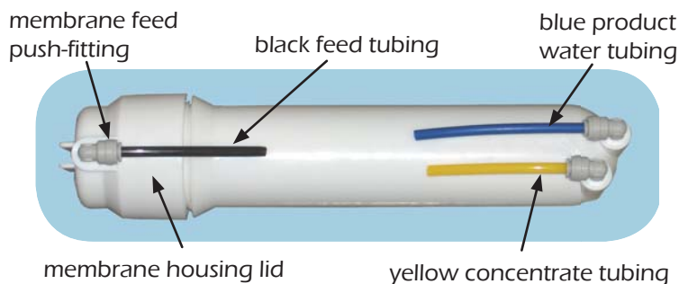
Tubing Connections to Membrane
