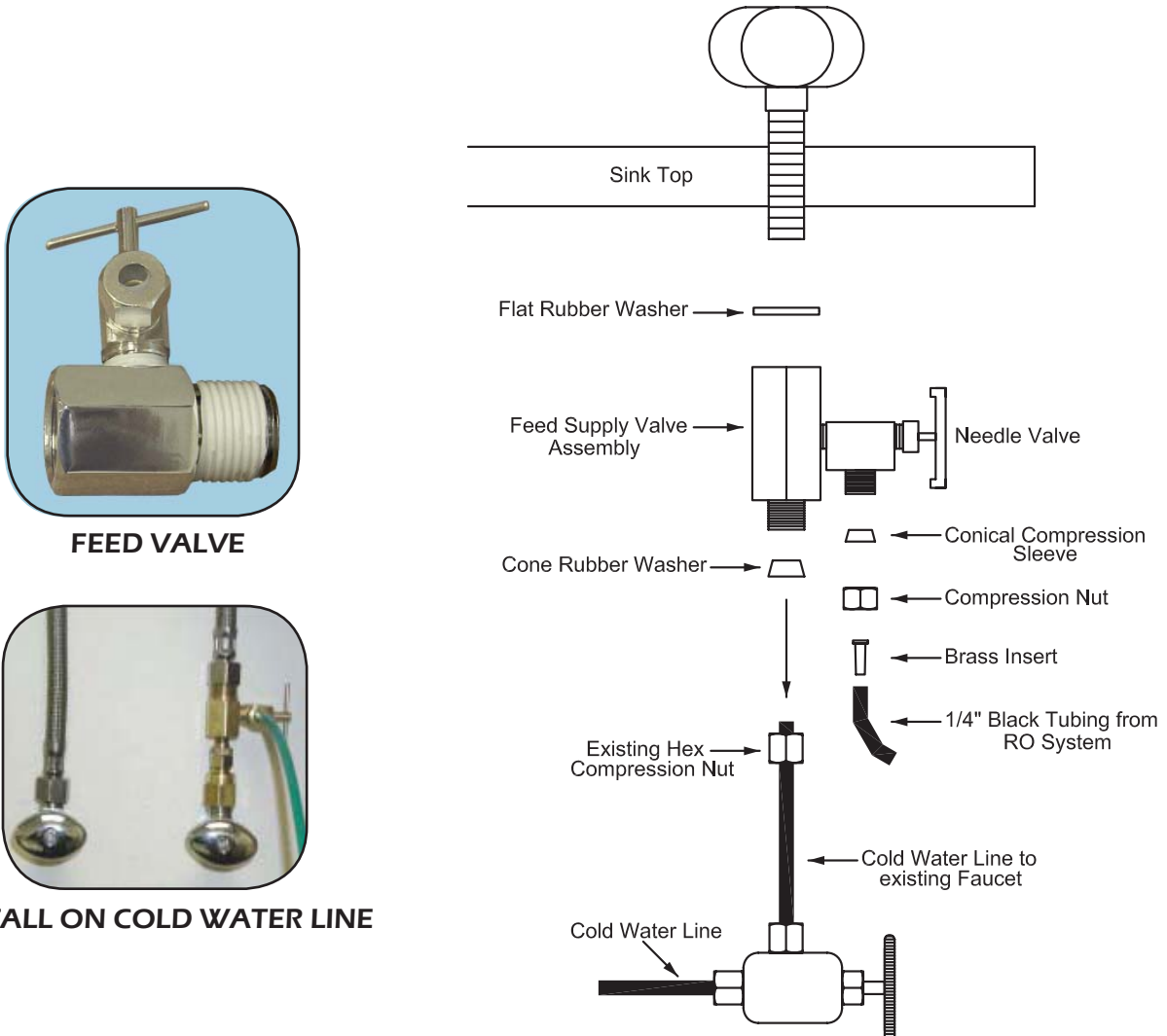
FIGURE 1: FEED SUPPLY INSTALLATION
