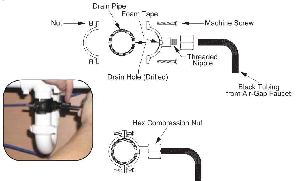
Figure 3: Drain Saddle Assembly Sequence
