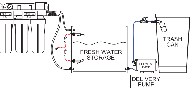
USE DELIVERY PUMP TO DELIVER WATER WHERE NEEDED FOR SALT MIXING OR TO SUMP
