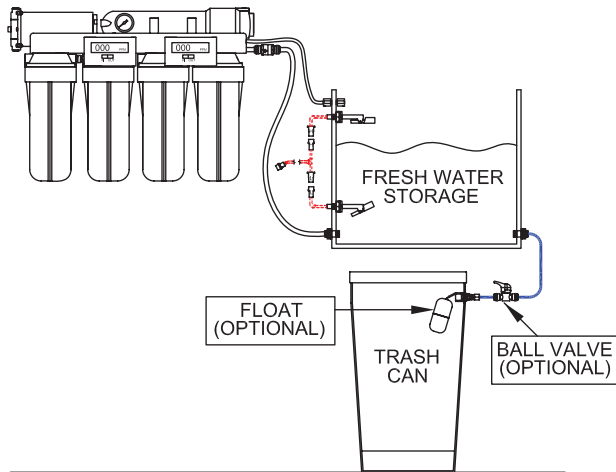
GRAVITY DRAIN WATER FROM ELEVATED TANK TO TRASH CAN FOR SALT MIXING OR TO SUMP
